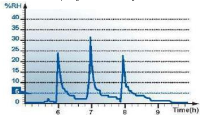
Progression of humidity level with 3 door openings of 30 seconds long
